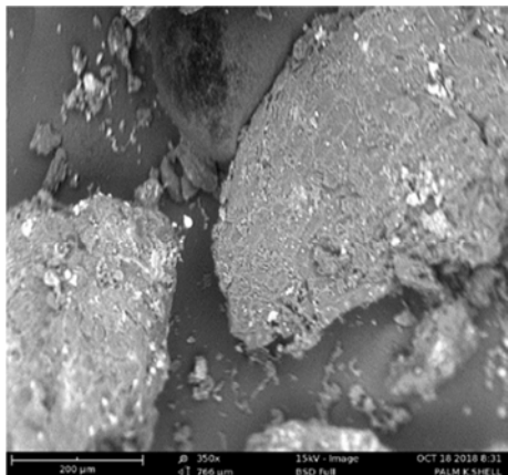
Figure 3. SEM micrograph of Palm Kernel Shell.
